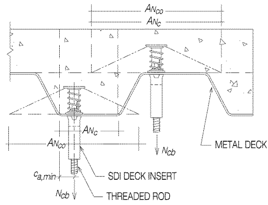
FIGURE 5 —IDEALIZATION OF CONCRETE ON DECK FOR DETERMINATION OF CONCRETE BREAKOUT STRENGTH IN ACCORDANCE WITH ACI 318
