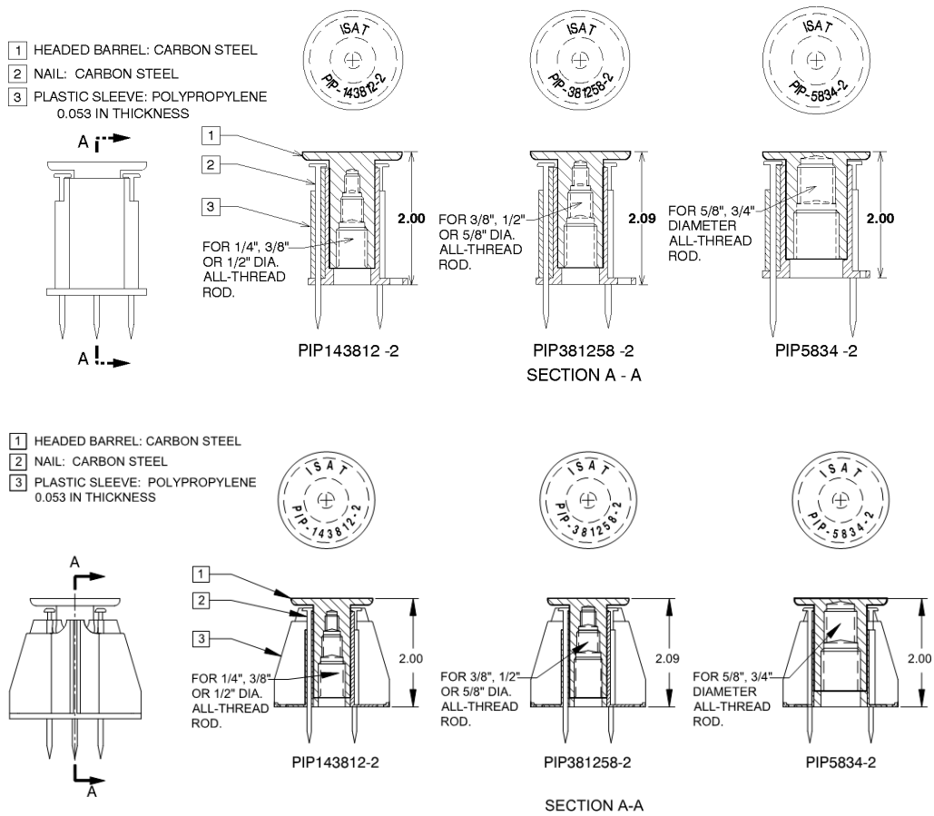
FIGURE 1—PIP CAST-IN-PLACE INSERTS FOR FORM POUR CONCRETE (TOP—STANDARD BASE; BOTTOM—WIDE BASE)
