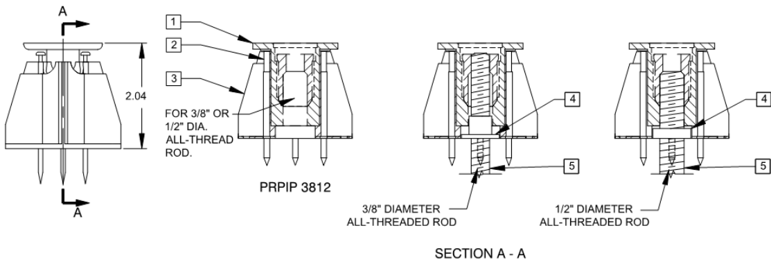
FIGURE 1B—PRPIP3812 CAST-IN-PLACE INSERTS FOR FORM POUR CONCRETE (TOP—STANDARD BASE; BOTTOM—WIDE BASE)
