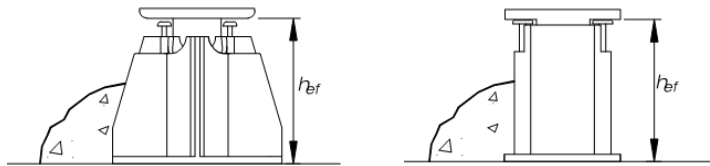
FIGURE 3—PIP AND ISAT-PRPIP3812 (PRPIP3812) INSERTS INSTALLED IN SOFFIT OF FORM POUR CONCRETE FLOOR AND ROOF ASSEMBLIES (LEFT—WIDE BASE; RIGHT—STANDARD BASE)
