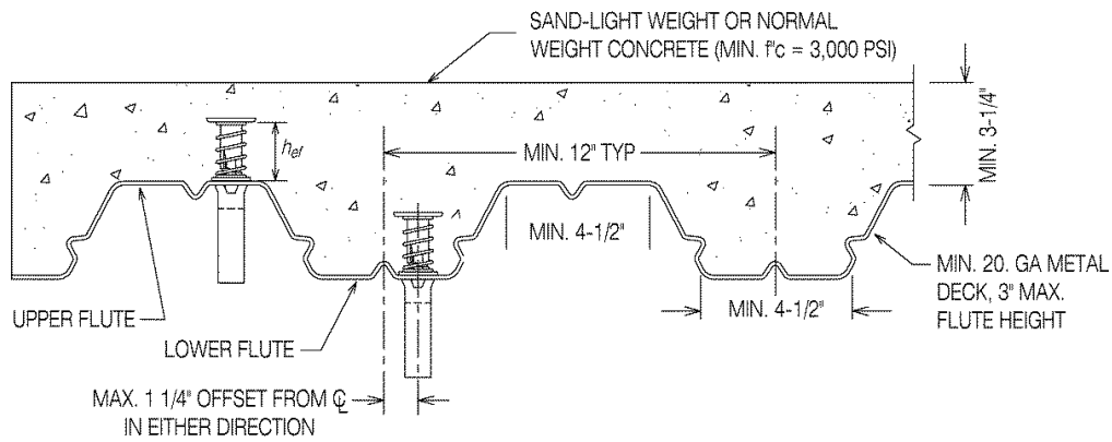
FIGURE 4—SDI INSERTS INSTALLED IN SOFFIT OF CONCRETE OVER METAL DECK FLOOR AND ROOF ASSEMBLIES 1,2,3,4
