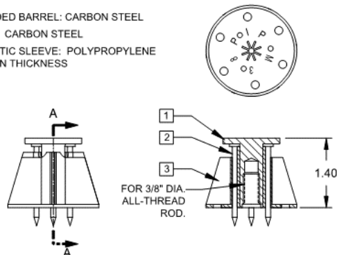
FIGURE 1C—PIM38 CAST-IN-PLACE INSERTS FOR FORM POUR CONCRETE
