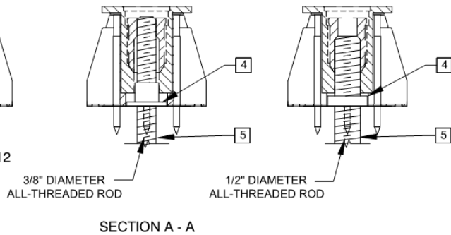
FIGURE 1A—ISAT-PRPIP3812 CAST-IN-PLACE INSERTS FOR FORM POUR CONCRETE (TOP—STANDARD BASE; BOTTOM—WIDE BASE)
