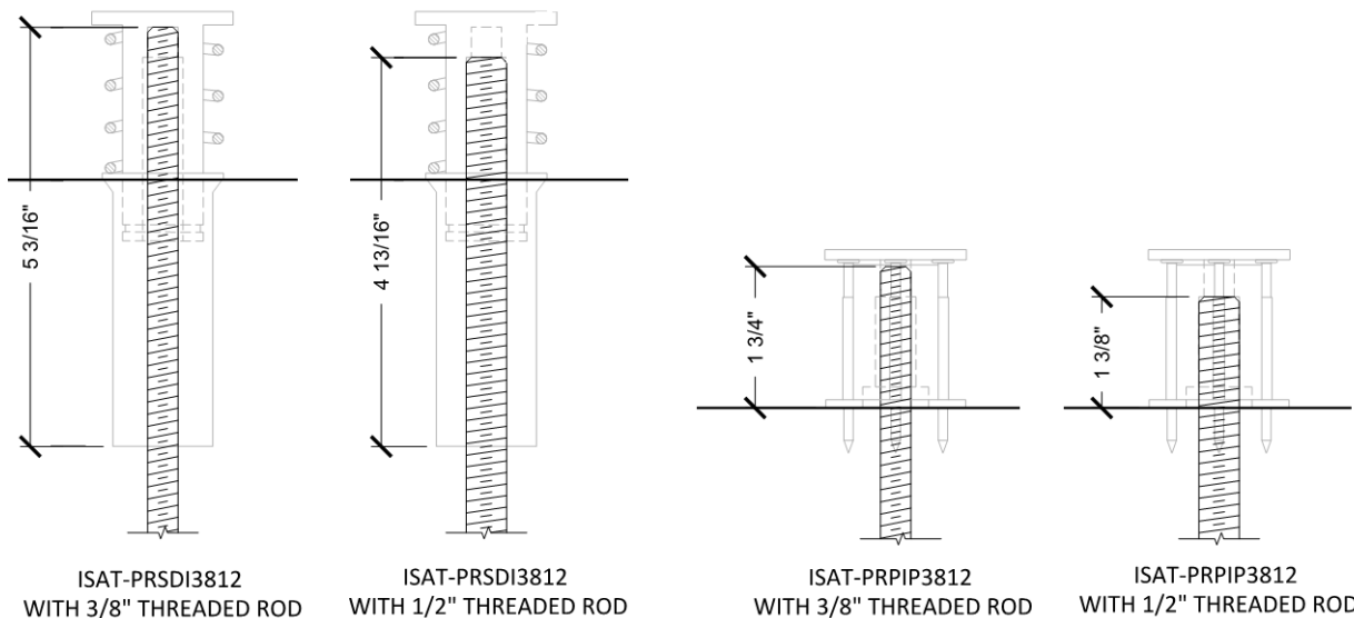
FIGURE 8 – REQUIRED THREADED ROD (ATR) ENGAGEMENT IN PUSH ROD INSERTS FOR PROPER INSTALLATION
