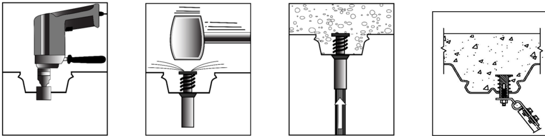
FIGURE 7—SDI INSTALLATION INSTRUCTIONS
