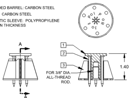
FIGURE 1B—PRPIP3812 CAST-IN-PLACE INSERTS FOR FORM POUR CONCRETE (TOP—STANDARD BASE; BOTTOM—WIDE BASE)
