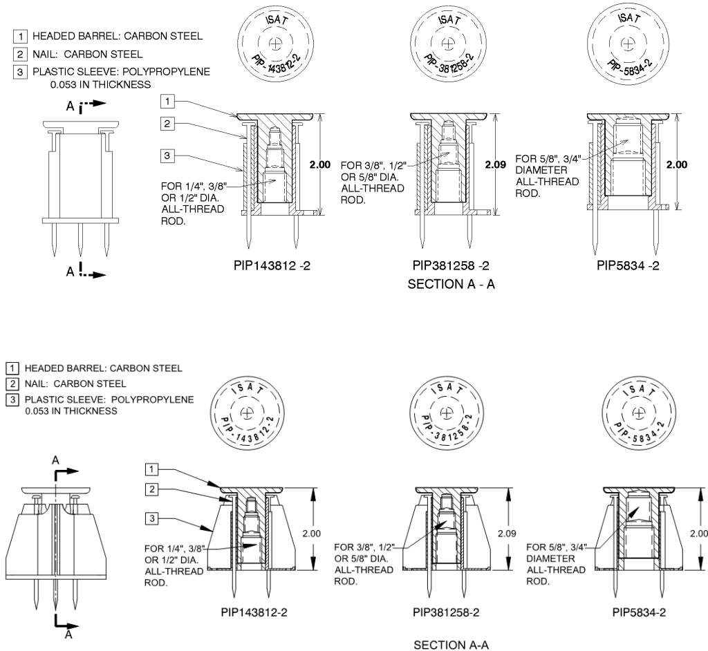
FIGURE 1—PIP CAST-IN-PLACE INSERTS FOR FORM POUR CONCRETE (TOP—STANDARD BASE; BOTTOM—WIDE BASE)
