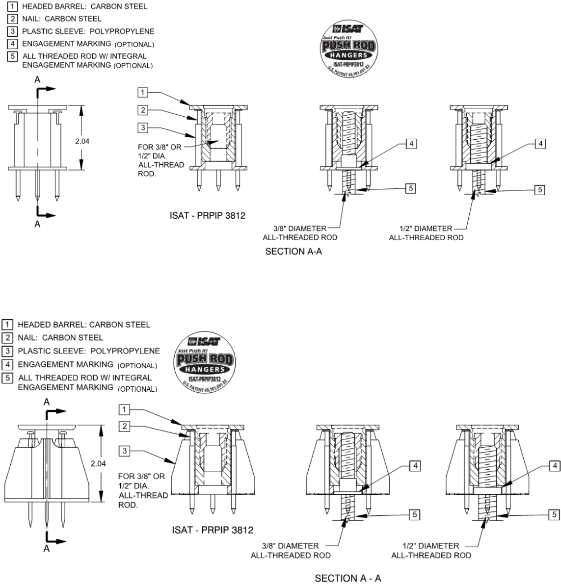
FIGURE 1A—ISAT-PRPIP3812 CAST-IN-PLACE INSERTS FOR FORM POUR CONCRETE (TOP—STANDARD BASE; BOTTOM—WIDE BASE)
