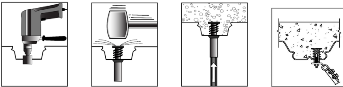
FIGURE 7—SDI INSTALLATION INSTRUCTIONS
